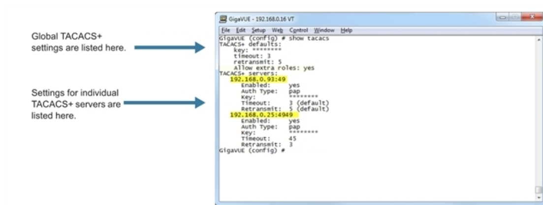
Figure 29 Results of show tacacs Command
