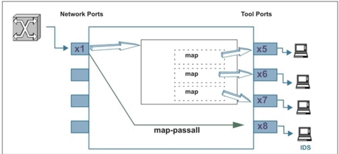
Figure 5 Sending All Traffic to IDS
