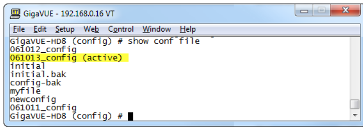
Figure 4 Showing Configuration Files
